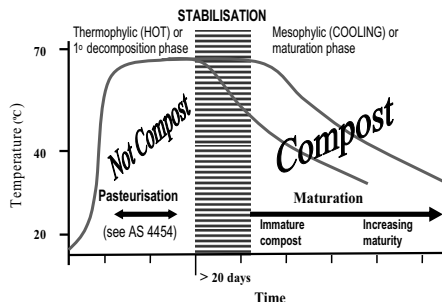
Figure1. Diagrammatic depiction of temperature change during 'in-vessel' or 'static pile' composting process.
