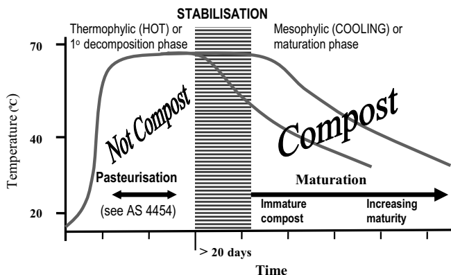
Figure 1. Diagrammatic depiction of an in-vessel composting process.
